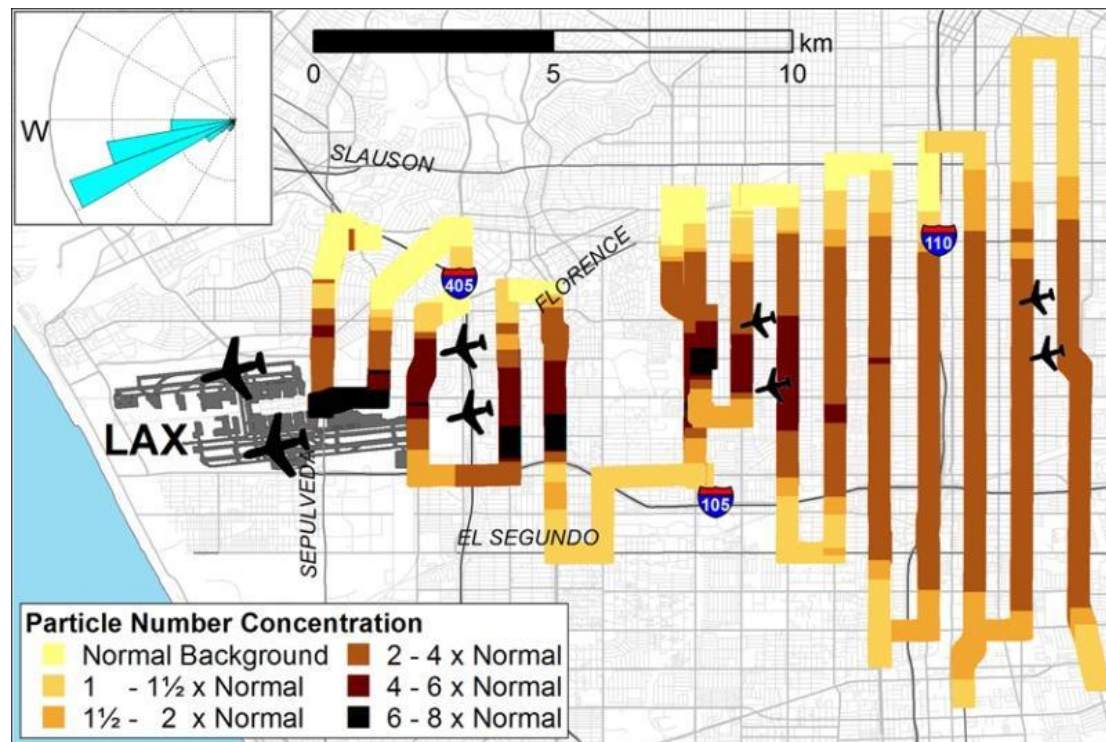
Figure 11 - Measured particle concentrations around LAX
