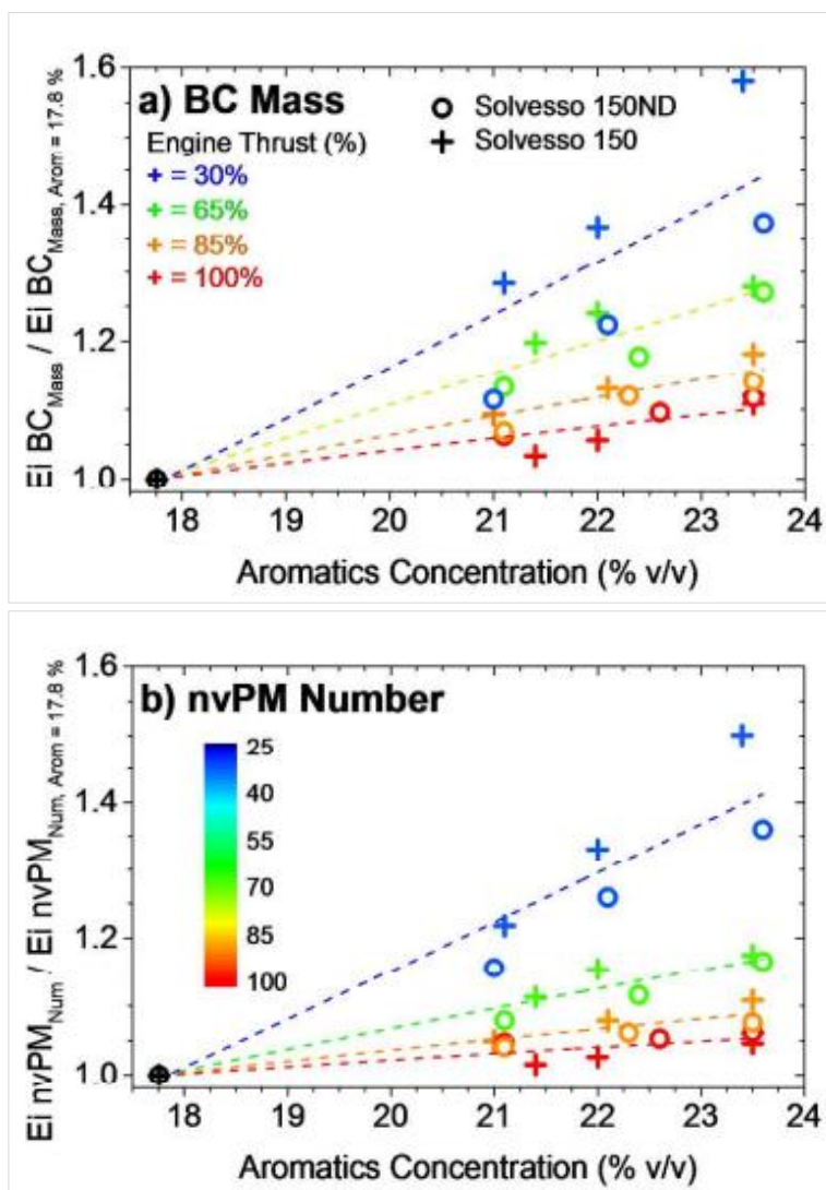
Figure 8 - Measurements of BC mass and nvPM number in the emissions of burning Jet A-1 fuel injected with aromatic solvent with naphthalene (Solvesso 150) and without naphthalene (Solvesso 150ND).
